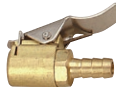
A107-7 (BRASS) A107-7-2 (ZINC) NO BLOCKING CHUCK FOR CAR A107-7-1 (BRASS) BLOCKING CHUCK FOR CAR SIZE: □1/4H □5/16H
